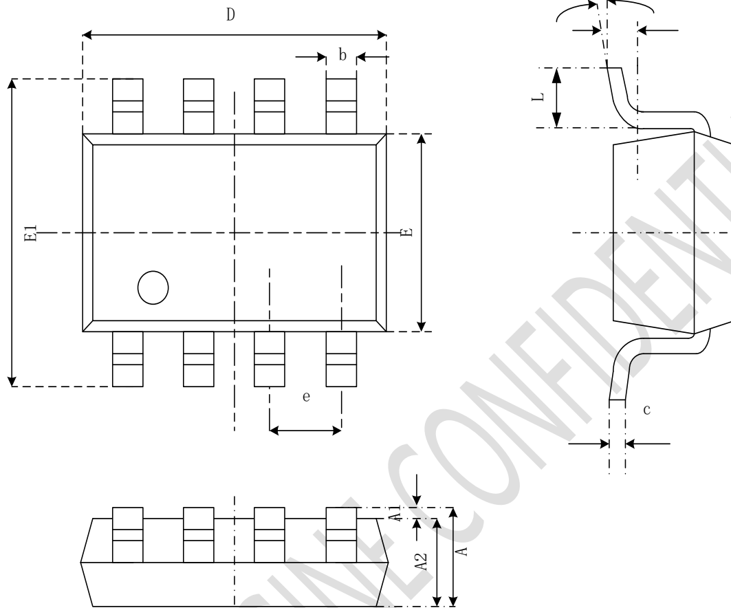
SOP8 PACKAGE OUTLINE DIMENSIONS
