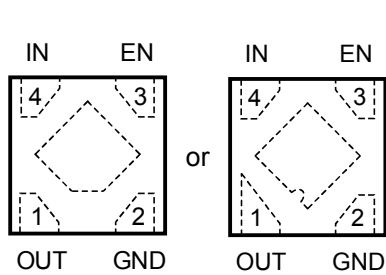
DFN1×1-4 (SK6513SD4)
