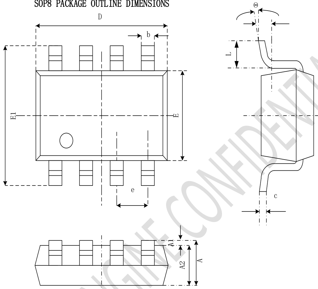
SOP8 PACKAGE OUTLINE DIMENSIONS
