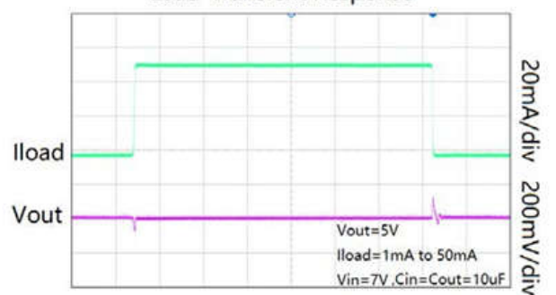
Load-Transient Response
