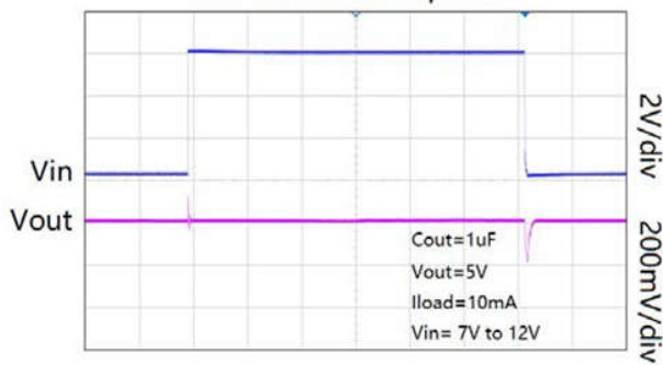
Line-Transient Response
