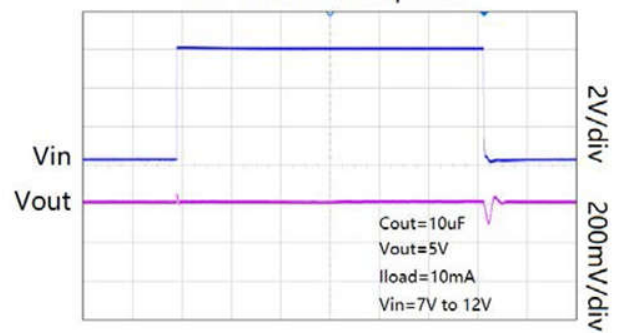
Line-Transient Response
