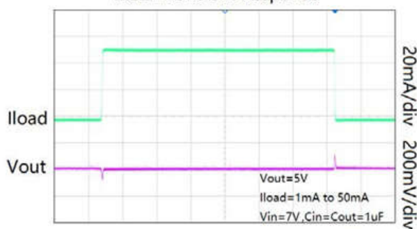
Load-Transient Response
