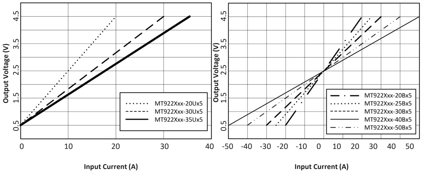
Figure.3 Output Voltage vs. Input Current
