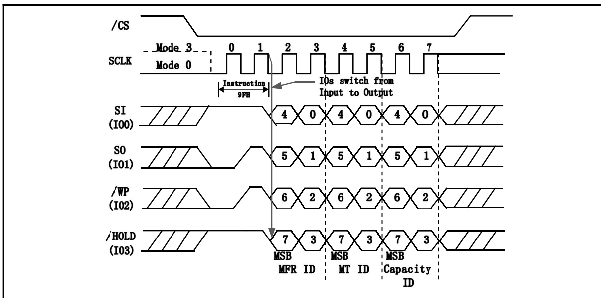
Figure 110. JEDEC ID Sequence Diagram (QPI Mode)
