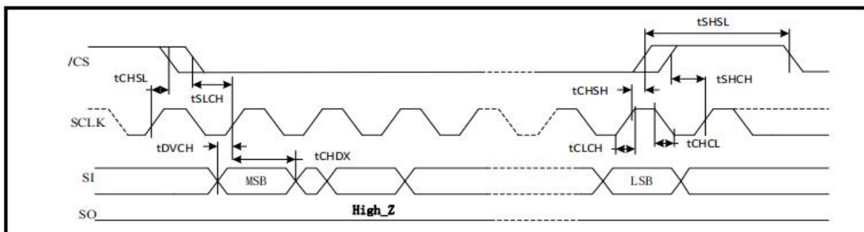
Figure 217. Output Timing
