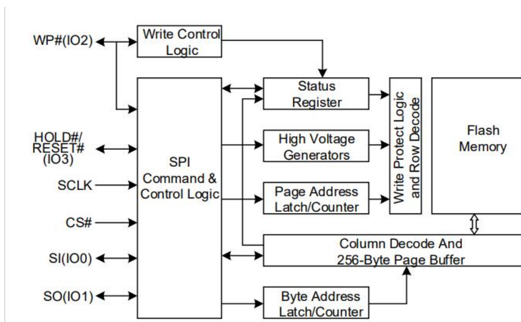
Figure 1. Logic diagram
