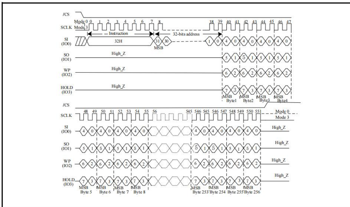
Figure 142. Quad Page Program Sequence Diagram (SPI Mode only/4-Byte Address Mode)
