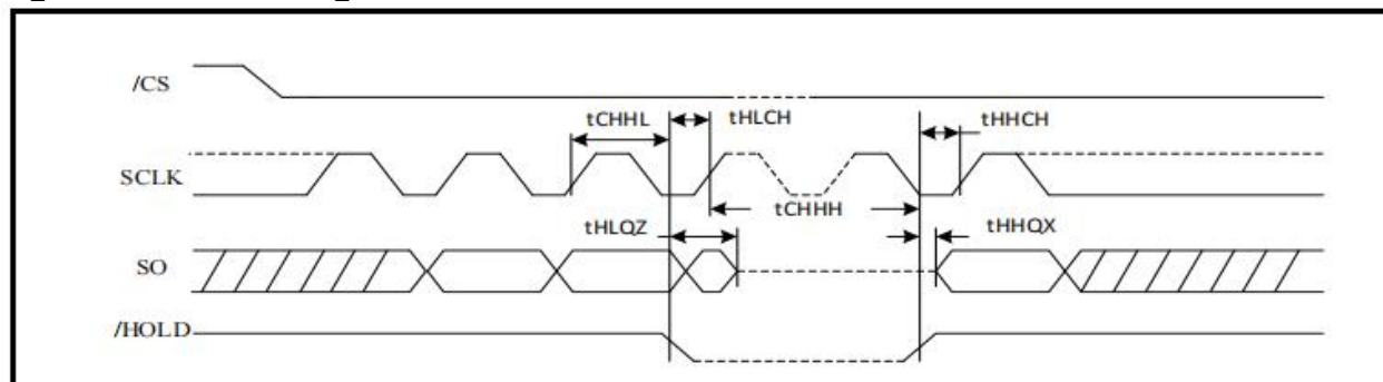
Figure 218. Hold Timing
