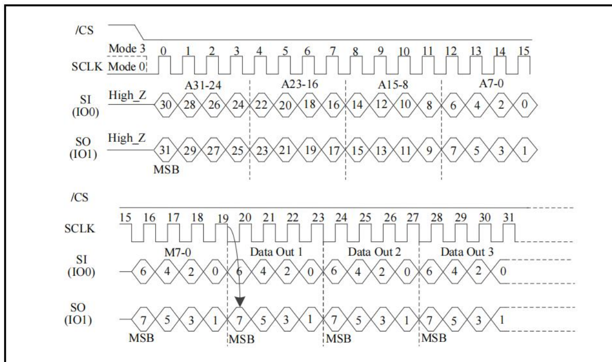
Figure 61. Dual I/O Fast Read Sequence Diagram (SPI Mode/4-Byte Address Mode; Previous instruction set (M5-4) =(1,0))
