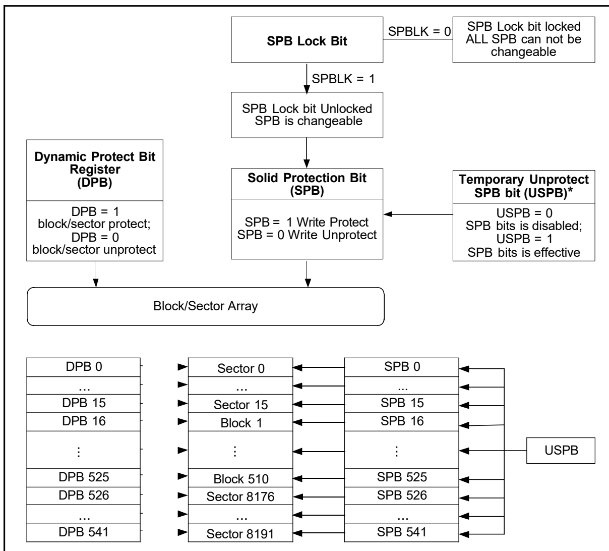
Figure 11. Single Die ZD25Q512 SPB, DPB and USB protection for Block/Sector Array
