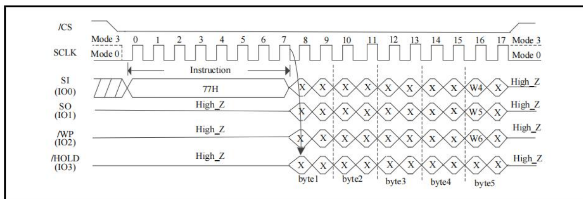
Figure 97. Set Burst with Wrap Sequence Diagram (SPI Mode only/4-Byte Address Mode)
