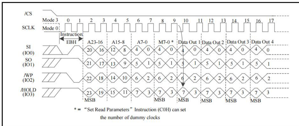
Figure 73. Quad I/O Fast Read Sequence Diagram (QPI Mode/4-Byte Address Mode; Initial instruction or previous ( M5-4 \neq (1,0) ))
