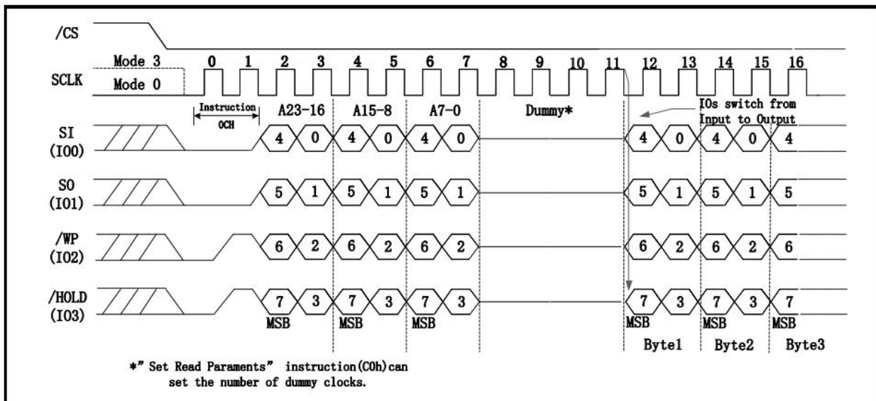
Figure 99. Burst Read with Wrap (QPI Mode only/3-Byte Address Mode)
