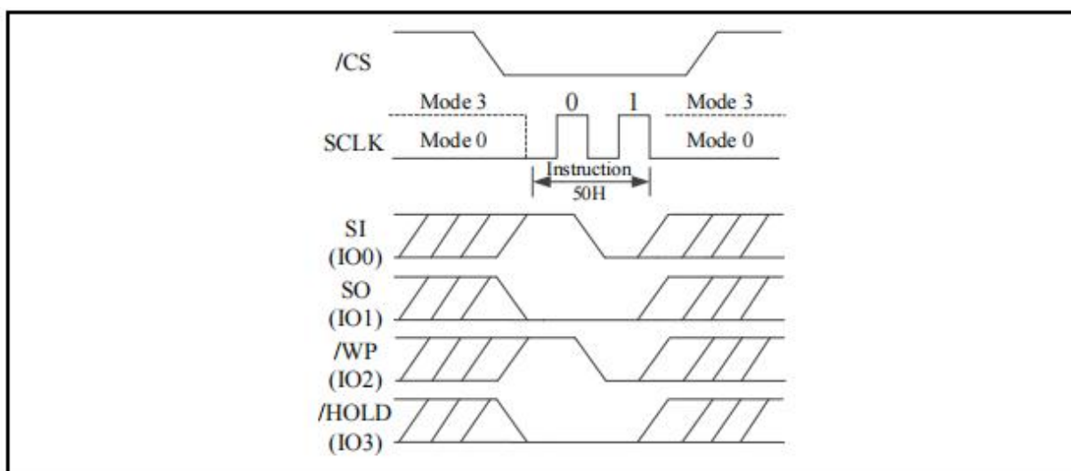
Figure 19. Write Enable for Volatile Status Register (QPI Mode)
