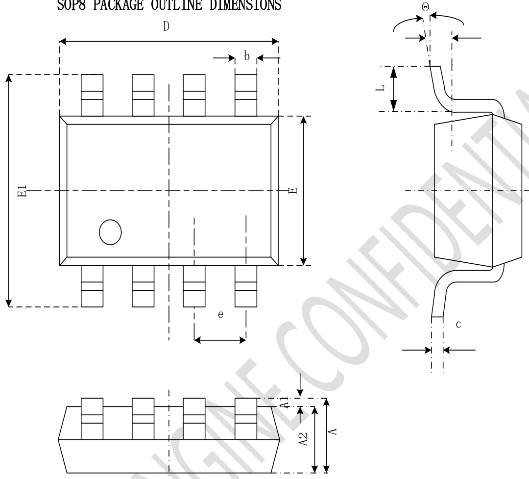
SOP8 PACKAGE OUTLINE DIMENSIONS
