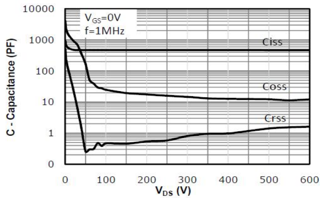
Fig 11: Capacitance Characteristics
