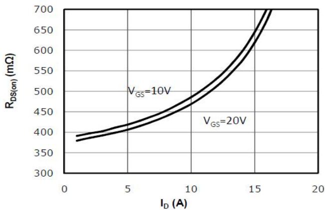
Fig 5: R_{DS(on)} Vs I_{DS} Characteristics ( T_C=25^\circ\text{C} )
