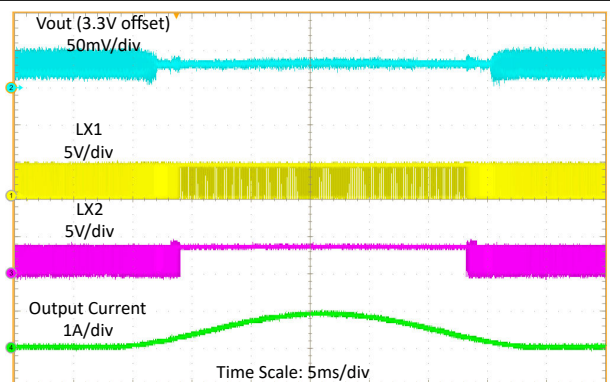
Figure 9-19. Load Sweep at 4.3-V Input Voltage
