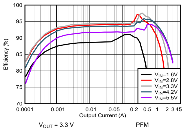
Figure 9-4. Efficiency vs Input Voltage (PFM)
