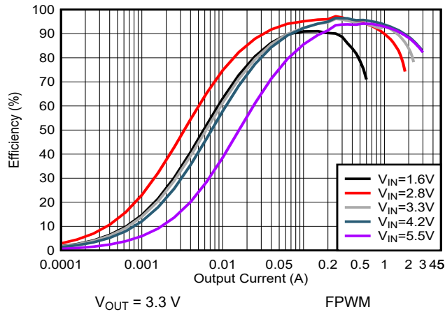
Figure 9-2. Efficiency vs Output Current (FPWM)
