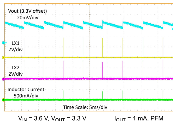
Figure 9-11. Switching Waveforms at 1-mA Load
