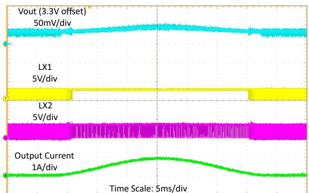
Figure 9-15. Load Sweep at 2.7-V Input Voltage
