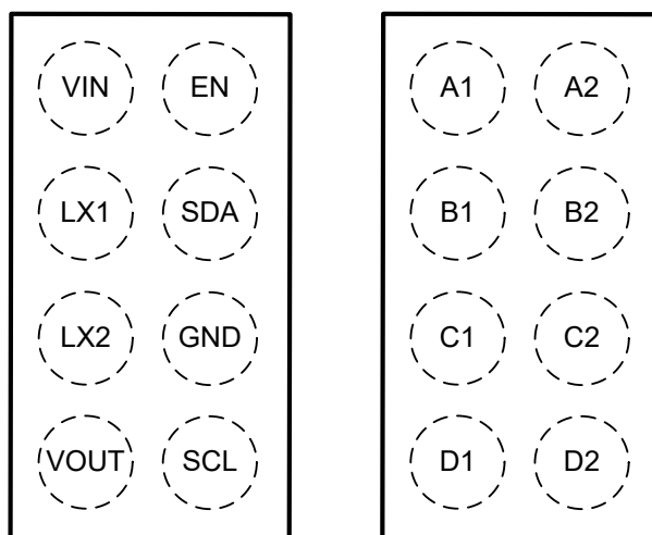
Figure 6-1. 8-Pin YBG WCSP Package (Top View)
