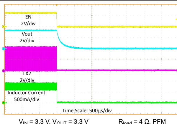
Figure 9-13. Shutdown by EN
