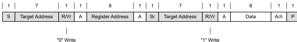
Figure 8-8. “Write” Data Transfer Format in Standard, Fast, and Fast-Plus Modes
