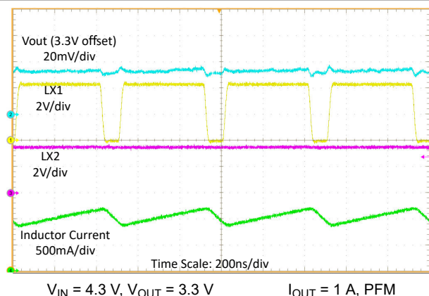
Figure 9-10. Switching Waveforms, Buck Operation with 1-A Load
