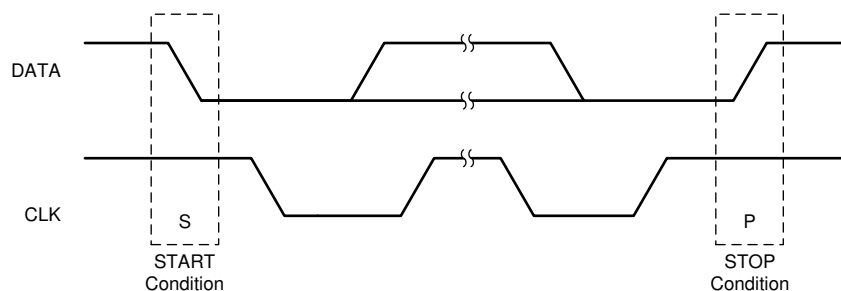
Figure 8-4. START and STOP Conditions
