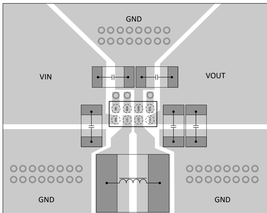
Figure 9-24. Layout Example
