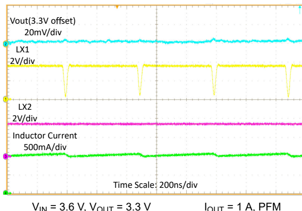
Figure 9-9. Switching Waveforms, Buck Operation with 1-A Load
