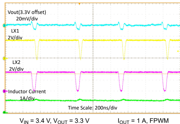
Figure 9-8. Switching Waveforms, Buck-Boost Operation with 1-A Load
