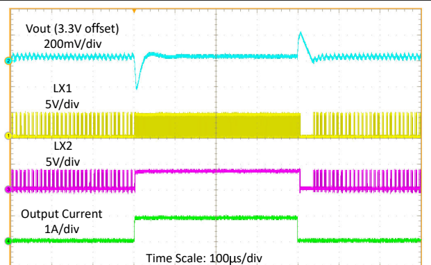
Figure 9-16. Load Transient at 3.6-V Input Voltage
