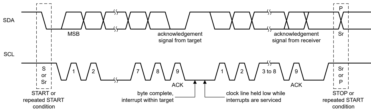
Figure 8-7. Bus Protocol
