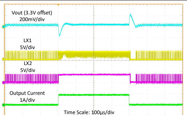
Figure 9-14. Load Transient at 2.7-V Input Voltage
