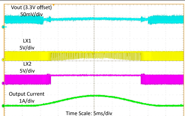
Figure 9-17. Load Sweep at 3.6-V Input Voltage
