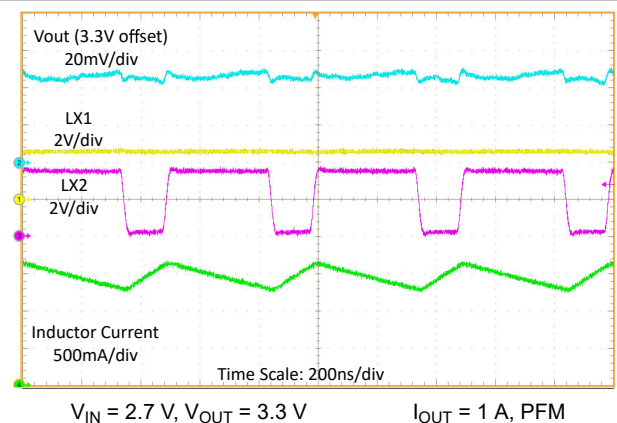
Figure 9-7. Switching Waveforms, Boost Operation with 1-A Load
