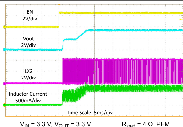
Figure 9-12. Start-Up by EN (Measured on TPS631013)
