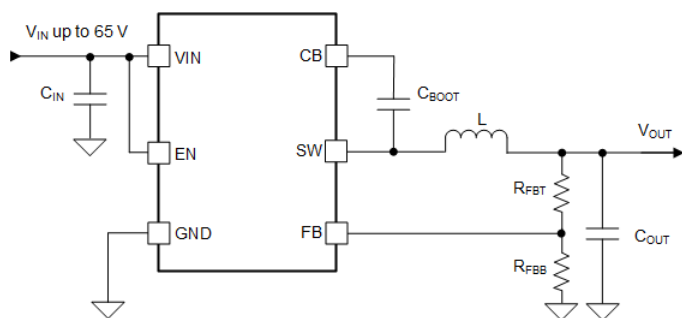
Simplified Schematic
