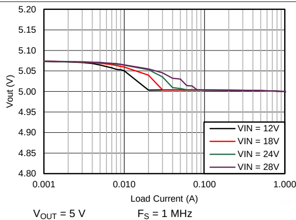
Figure 67. Output Voltage Regulation
