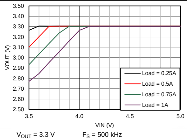
Figure 50. Dropout Curve
