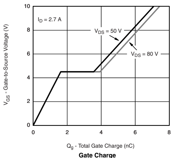
I_D = 2.7\text{ A} V_{DS} = 50\text{ V} V_{DS} = 80\text{ V} Q_g - Total Gate Charge (nC) Gate Charge
