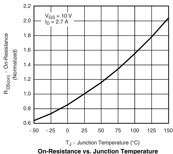
V_{GS} = 10\text{ V} I_D = 2.7\text{ A} T_J - Junction Temperature ( ^\circ\text{C} ) On-Resistance vs. Junction Temperature
