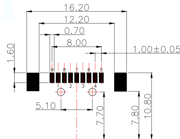
REFERENCE PCB LAYOUT
