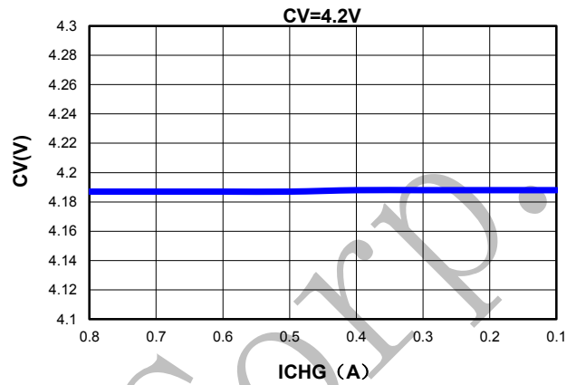
Chart 2 CV vs. ICHG@VIN=5V
