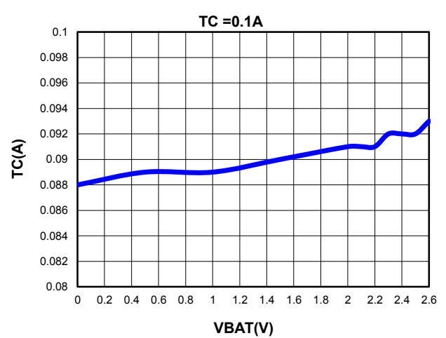
Chart 6 TC vs. VBAT@VIN=5V
