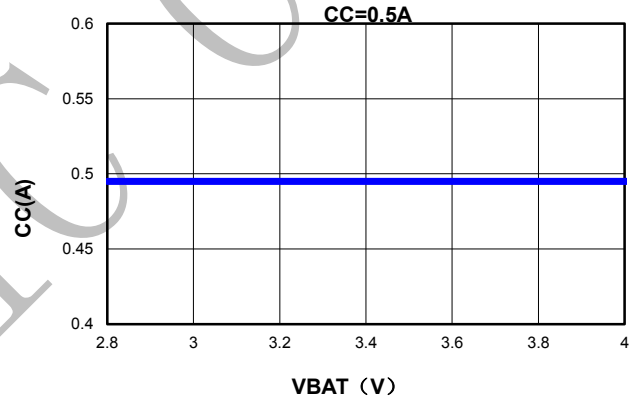
Chart 4 CC vs. VBAT@VIN=5V
