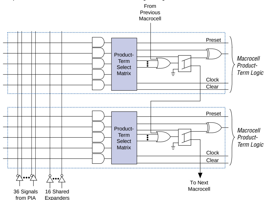
Figure 6. Parallel Expanders
