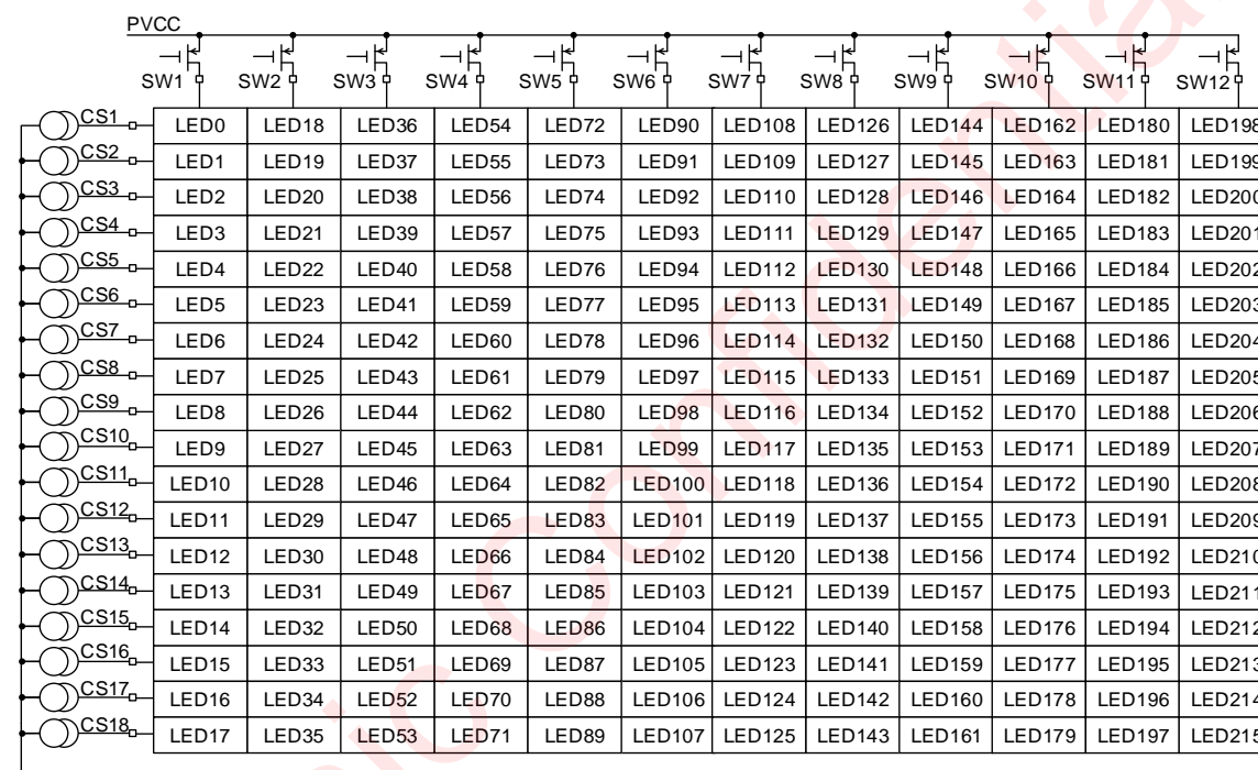
Figure 16 LED Location
