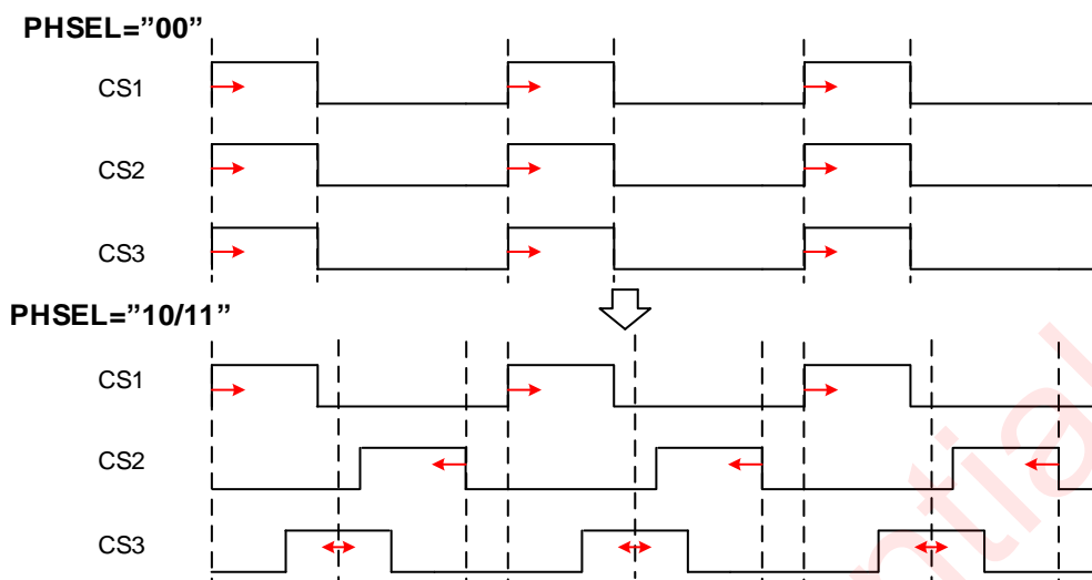
Figure 22 Three-Phase Mode
