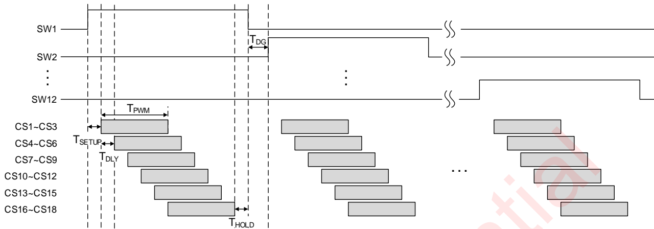
Figure 19 Scanning Timing
