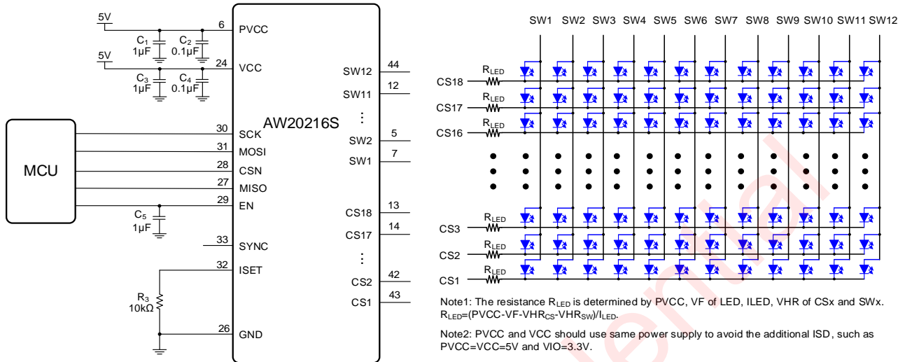
Figure 1 AW20216S Application Circuit
