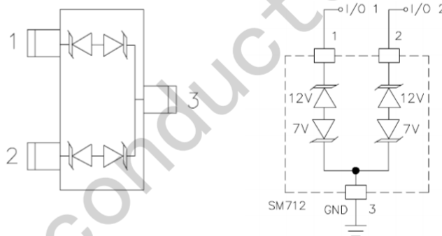
SOT23 (Top View)
