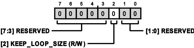
Figure 87. Address: 0x0F, Reset: 0x00, Name: LOOP_CONFIG_B
