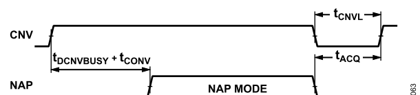
Figure 62. Nap Mode Timing for the AD4858
