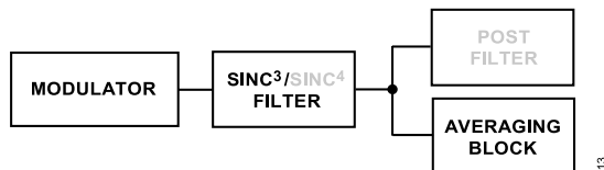
Figure 103. Fast Settling Mode, \text{Sinc}^3 + \text{Sinc}^1 Filter
