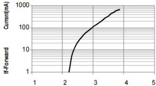
Fig.2-Forward Current vs. Forward Voltage
