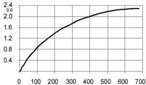
Fig.1-Relative Luminous Intensity vs. Forward Current
