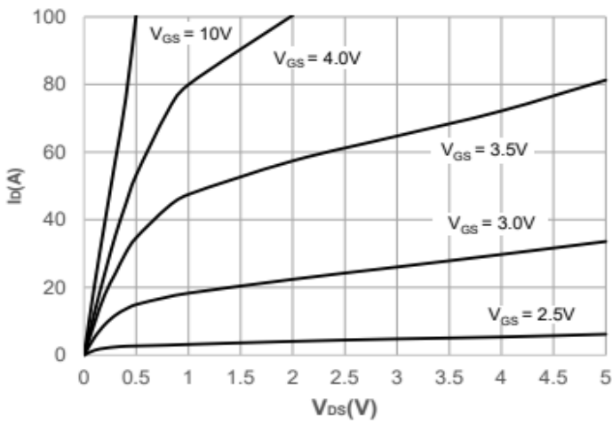
Output Characteristics
