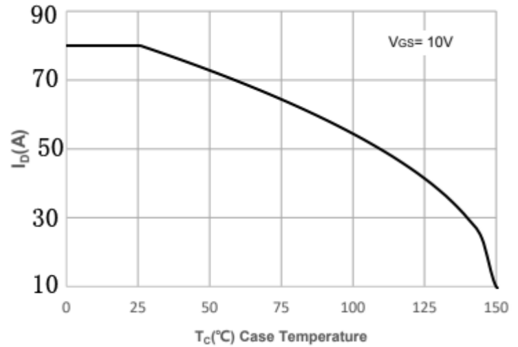
Case Temperature
