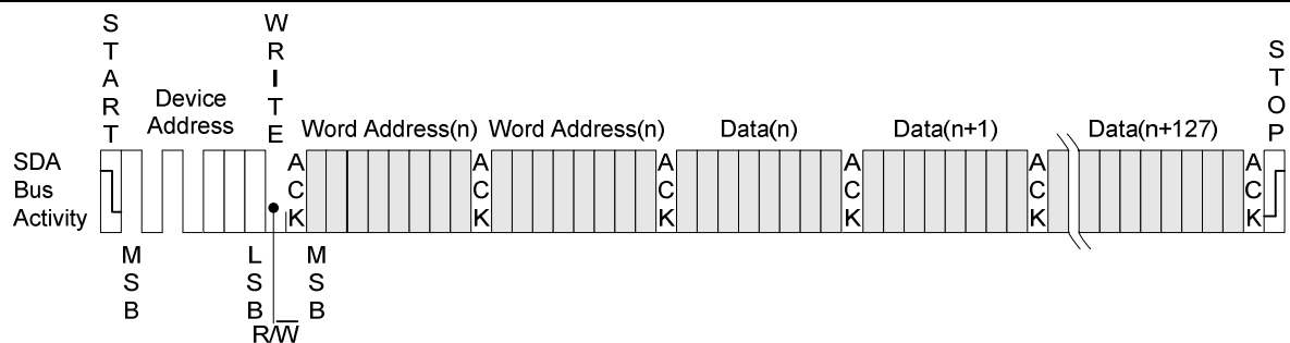
Figure 1-7. Page Write
