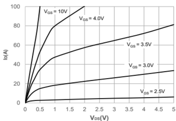
Output Characteristics
