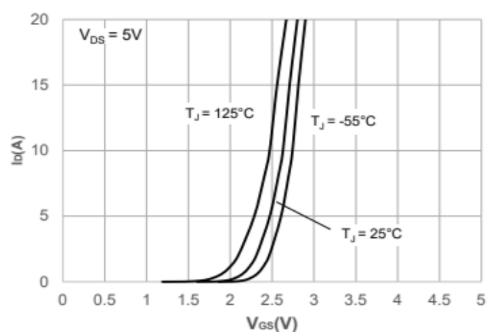
Typical Transfer Characteristics
