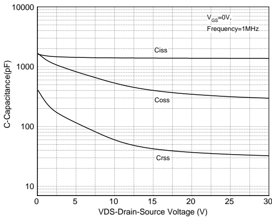
Figure 9: Capacitance Characteristics
