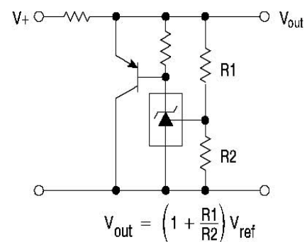
Higher-current Shunt
