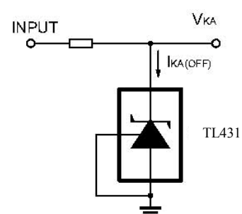
Test Circuit For I_{KA}(\text{OFF})
