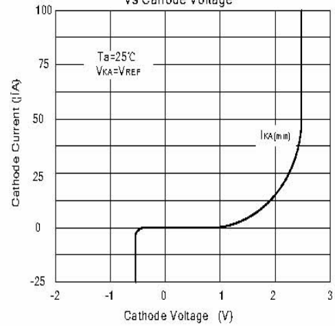
Fig 2 Cathode Current Vs Cathode Voltage
