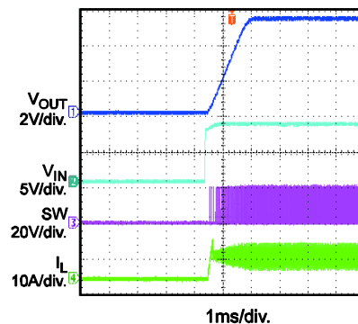
Transient
