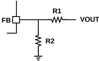
Figure 6: Feedback Network
