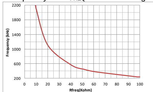
Figure 3: Switching Frequency vs R_{FREQ}
