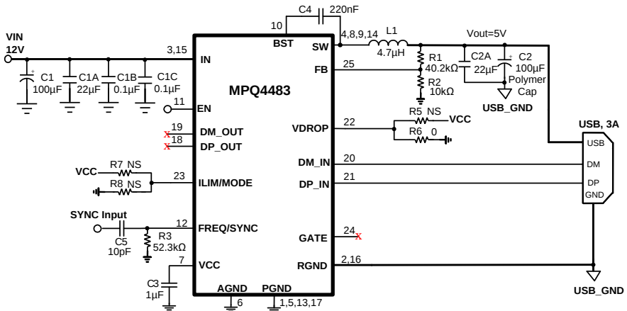
Figure 9: V_{IN}=12V , V_{OUT}=5V , I_{OUT}=3A , DCP Mode, Without GND Short to Battery Protection
