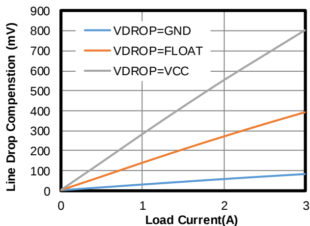
Line Drop Compensation vs. Load Current
