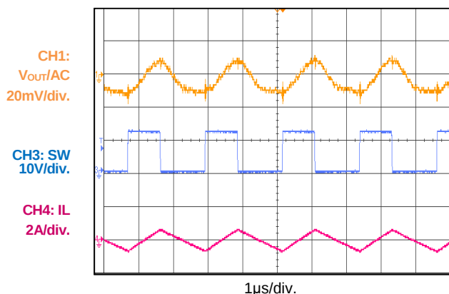
Output Ripple
