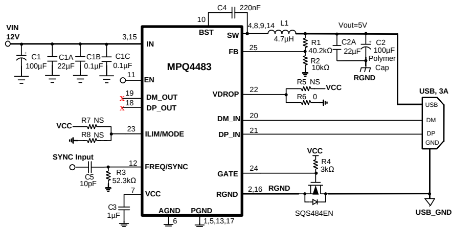
Figure 8: V_{IN}=12V , V_{OUT}=5V , I_{OUT}=3A , f_s=450KHz , DCP Mode, with GND Short to Battery Protection
