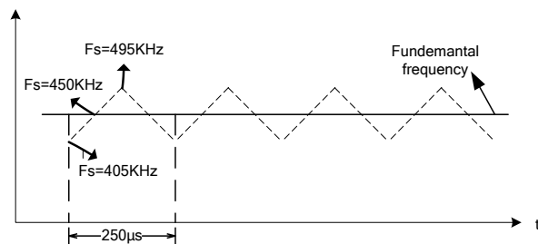
Figure 4: Frequency Spread Spectrum
