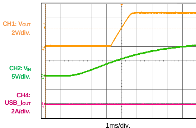
Power Start-Up
