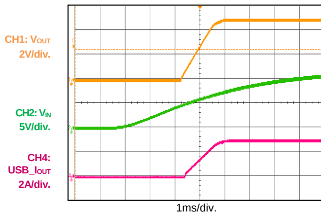
Power Start-Up
