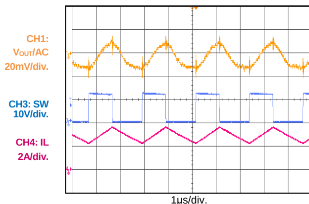
Output Ripple
