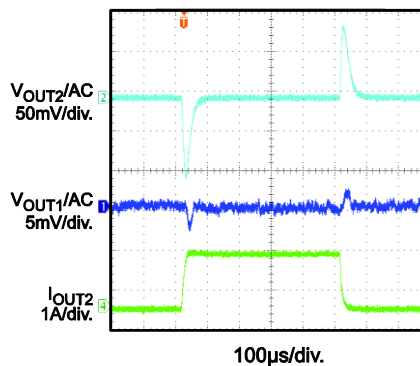
CH1 Steady State, CH2 Load Transient
