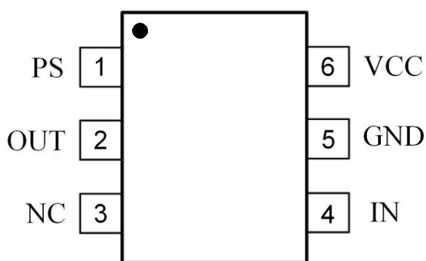
HBT191(SOT23-6)
