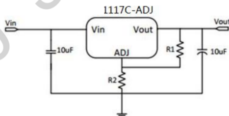
Application Circuit of SAMS1117-ADJ
