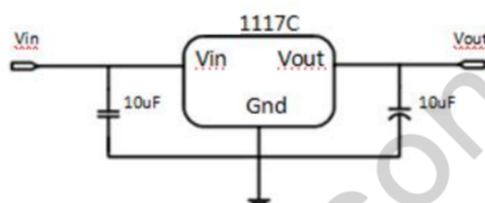
Application circuit of SAMS1117 fixed version
