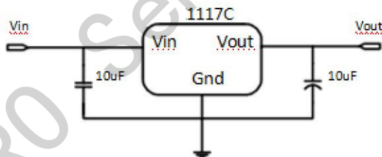
Application circuit of SAMS1117 fixed version
