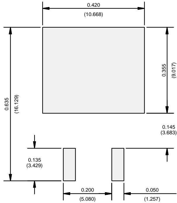
Recommended Minimum Pads Dimensions in Inches/(mm)
