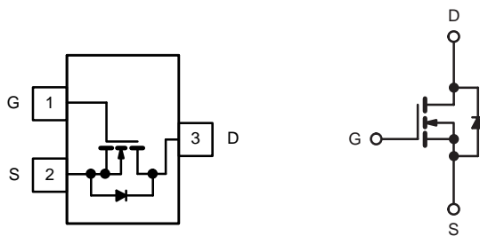
N-Channel MOSFET
