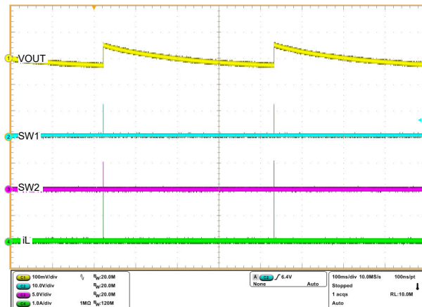
Figure 7-3. Switching Waveforms in V_{IN} = 12V , V_{OUT} = 5V , I_O = 0A , PFM
