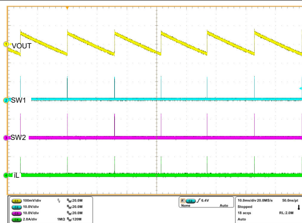
Figure 7-5. Switching Waveforms in V_{IN} = 12V , V_{OUT} = 12V , I_O = 0A , PFM
