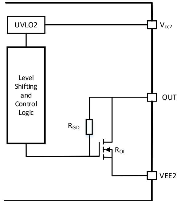
Figure 8.6 Active pulldown
