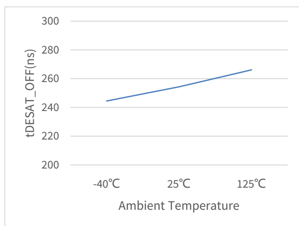
Figure 6.23 t_{\text{DESAT\_OFF}} vs Temperature
