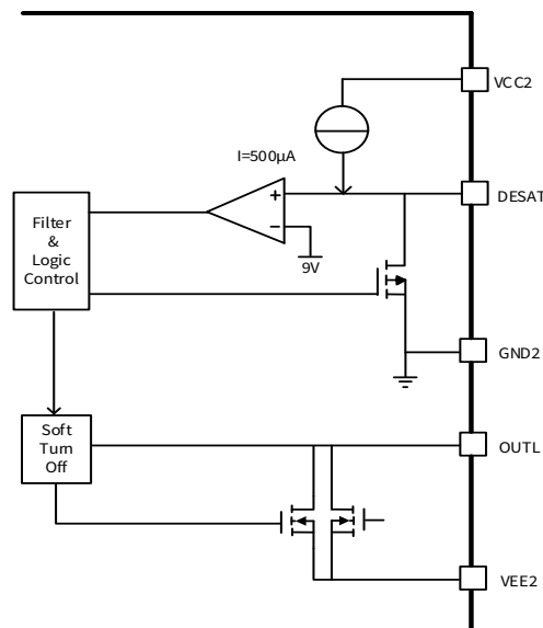
Figure 8.9 DESAT Protection
