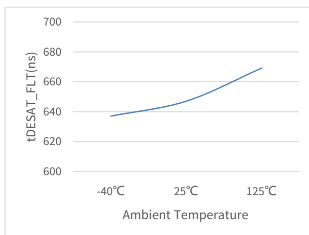
Figure 6.24 t_{\text{DESAT\_FLT}} vs Temperature
