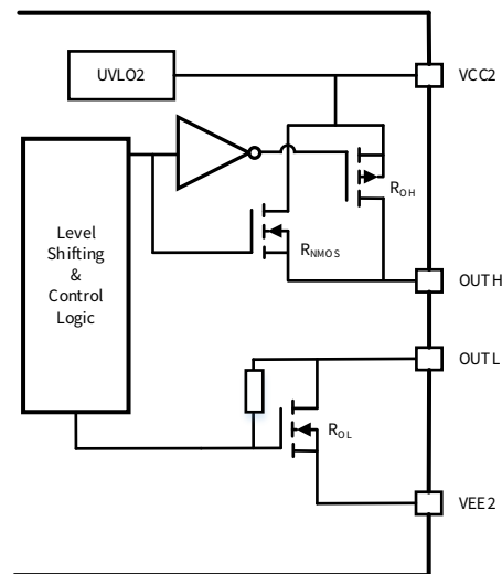
Figure 8.3 NSI66x1A output stage
