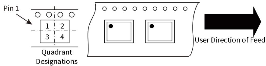
Figure 13.3 Quadrant Designation for Pin1 Orientation in Tape
