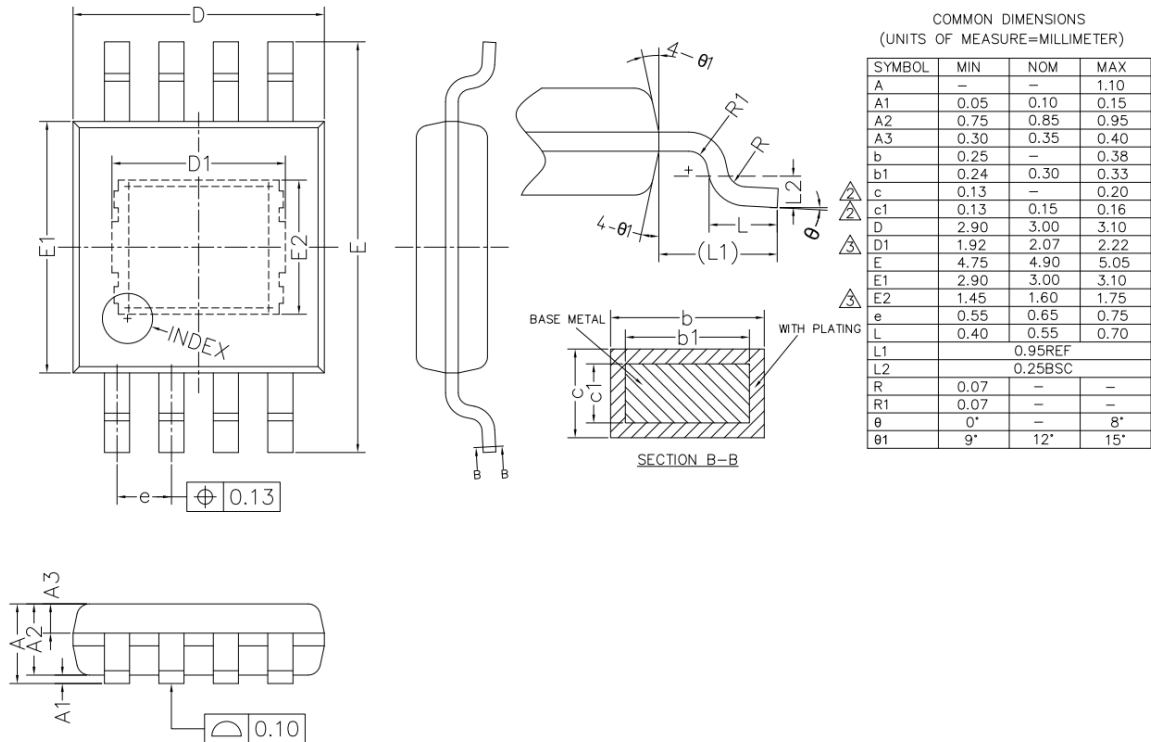
Figure 10.1 HMSOP-8 Package Shape and Dimension in millimeters
