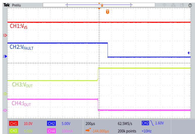
Figure 6.5 Open-Load Protection
