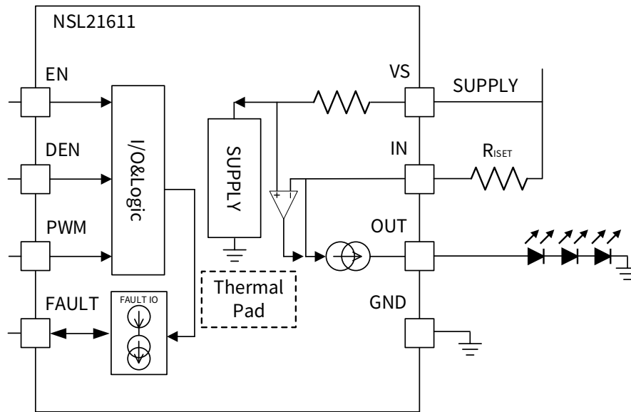
Figure 7.2 NSL21611 Block Diagram
