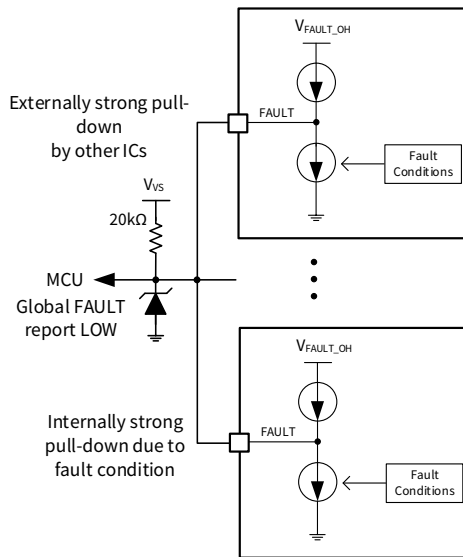
Figure 7.5 All off if one fails application
