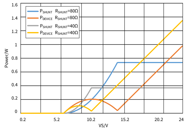
Figure 6.12 Power Dissipation vs Supply Voltage ( I_{set}=99mA )
