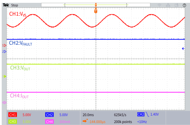
Figure 6.9 Superimposed Alternating Voltage 15Hz
