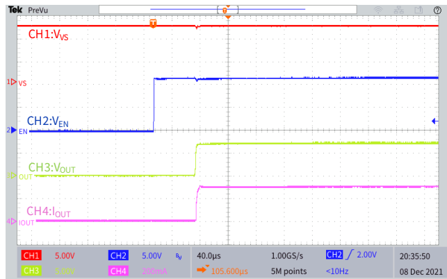
Figure 6.1 Start Up
