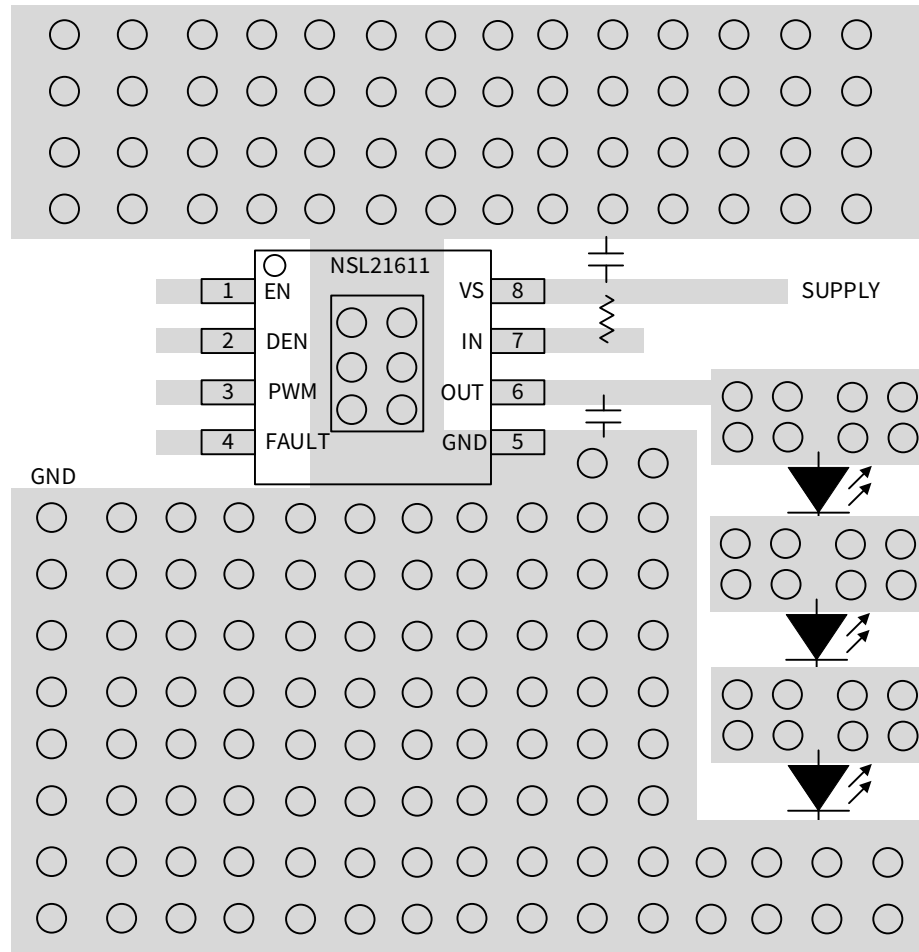
Figure 9.2 Example Layout Diagram for NSL21611
