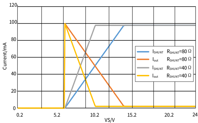
Figure 6.11 Output Current Distribution vs Supply Voltage ( I_{set}=99mA )
