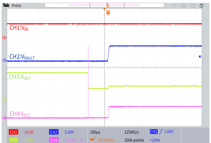
Figure 6.6 Open-Load Protection Recovery
