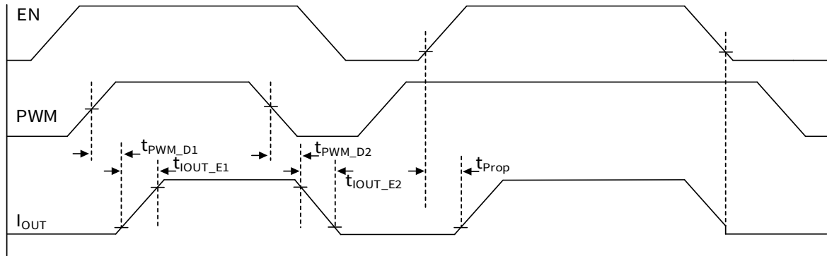
Figure 6.13 Start up sequence & PWM dimming timing
