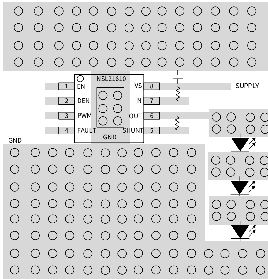
Figure 9.1 Example Layout Diagram for NSL21610
