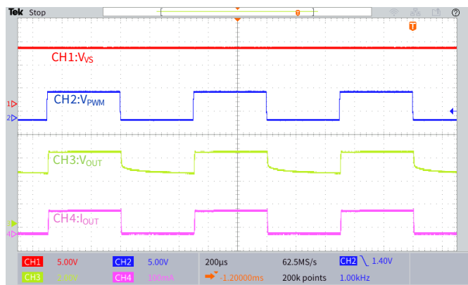
Figure 6.3 PWM Dimming at 1kHz
