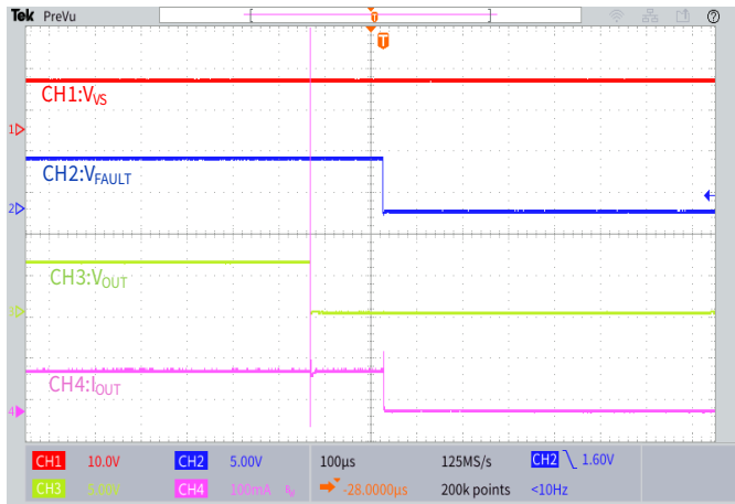
Figure 6.7 LED Short-to-GND Protection
