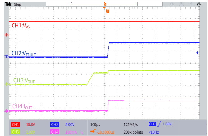
Figure 6.8 LED Short-to-GND Protection Recovery
