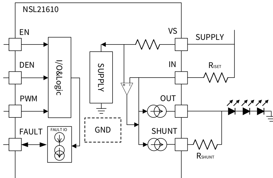
Figure 7.1 NSL21610 Block Diagram
