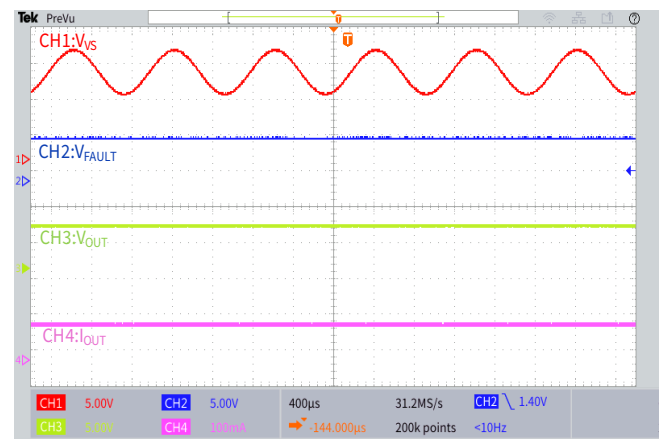
Figure 6.10 Superimposed Alternating Voltage 1kHz
