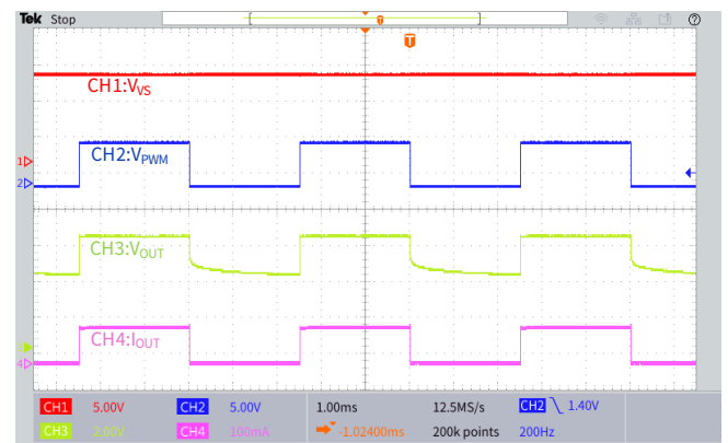
Figure 6.4 PWM Dimming at 200Hz
