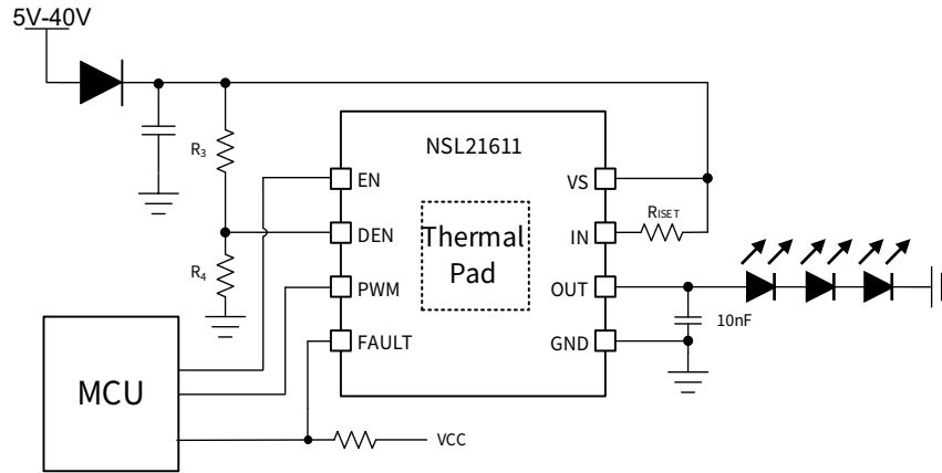
Figure 8.2 Application with MCU
