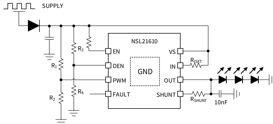
Figure 7.4 NSL21610 Power Supply Control LED Brightness Dimming
