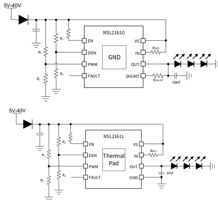
Figure 8.1 Simple Application Without MCU
