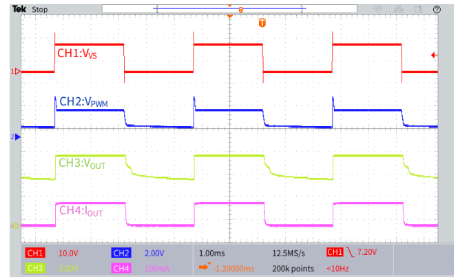
Figure 6.2 Power Supply Dimming at 200Hz
