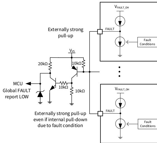
Figure 7.6 Others remain on if one fails application
