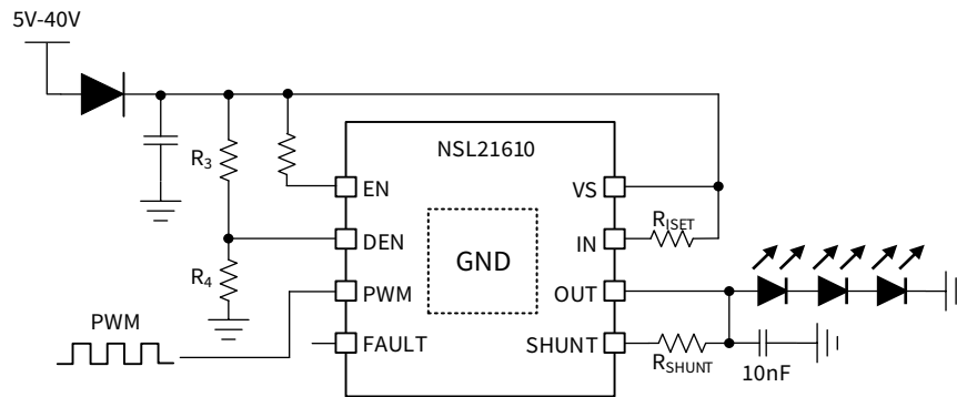
Figure 7.3 NSL21610 PWM Control LED Brightness Dimming
