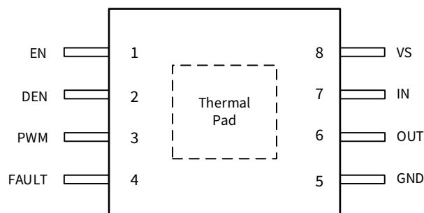
Figure 1.2 NSL21611 Package
