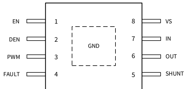
Figure 1.1 NSL21610 Package
