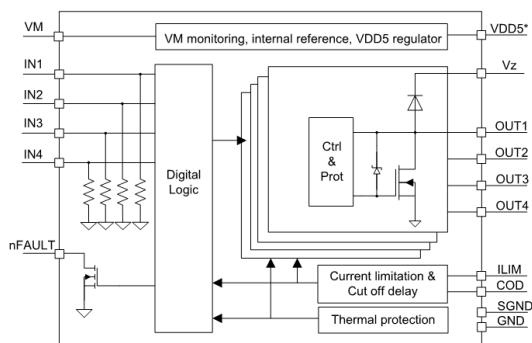
Figure 0.1 NSD5604E/ NSD5604NE Block Diagram
