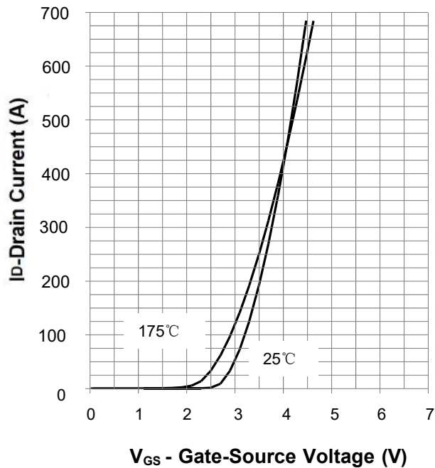
Transfer Characteristics
