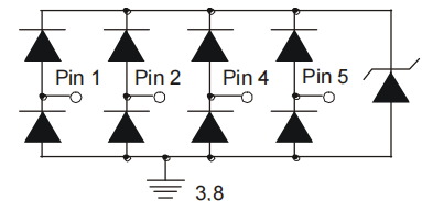
Device Schematic
