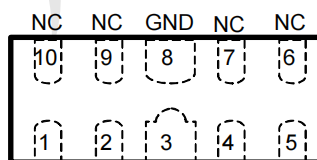
Pin Description (Top View)
