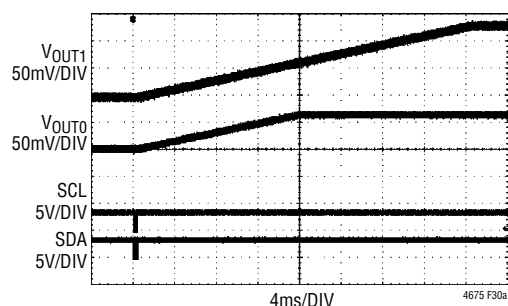
(30a) PMBus Operation (Req. 0x01): 0x80 → 0xA8 (Margin High)
