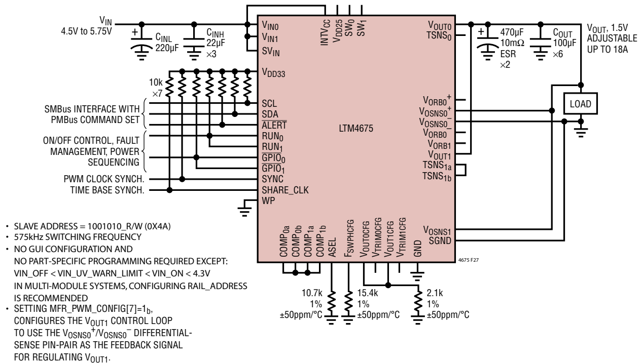
Figure 27. 1.5V Output DC/DC \mu Module Regulator with I²C/SMBus/PMBus Serial Interface
