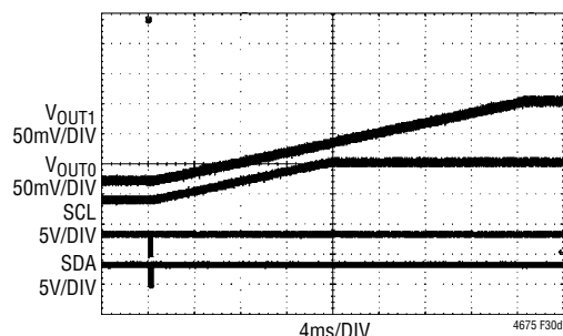
(30d) PMBus Operation (Req. 0x01): 0x98 → 0x80 (Margin Off)
