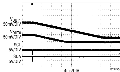
(30c) PMBus Operation (Req. 0x01): 0x80 → 0x98 (Margin Low)
