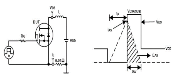
Fig11. Unclamped Inductive Test Circuit and waveform
