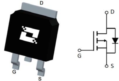
TO-252
