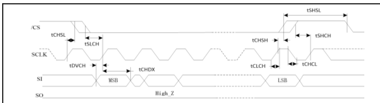
Figure 212. Output Timing
