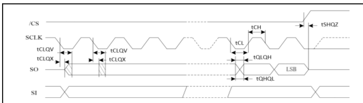
Figure 213. Hold Timing
