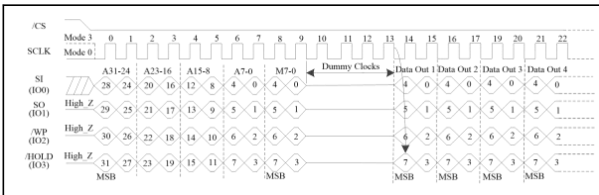
Figure 66. Quad I/O Fast Read Sequence Diagram (SPI Mode/4-Byte Address Mode; Initial instruction or previous (M5-4=(1,0)))
