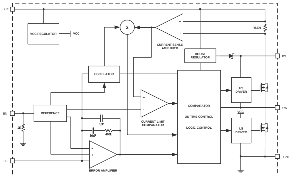
Figure 2. HE9427Block Diagram
