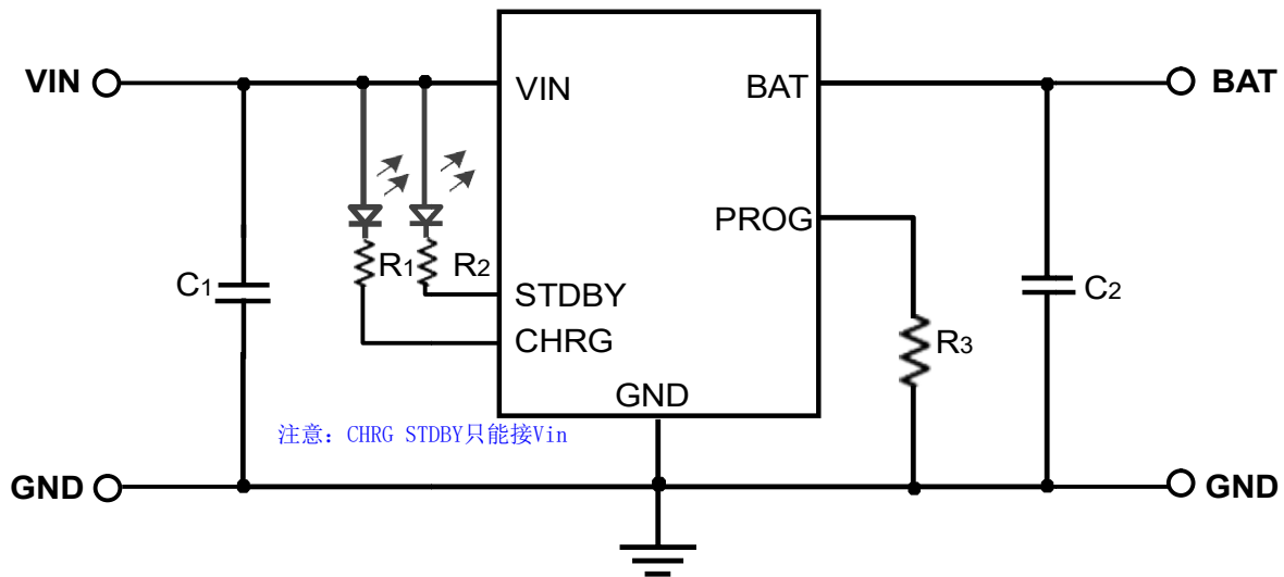
Figure 2. HE4064EB/HE4064EC/HE4064ED Typical Application Circuit
