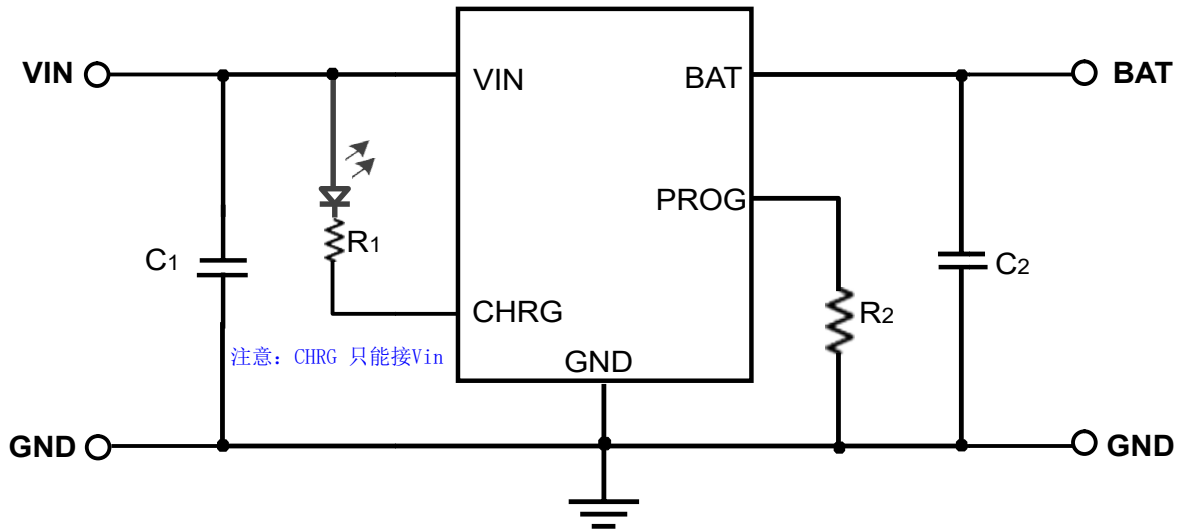
Figure 1. HE4064EA Typical Application Circuit
