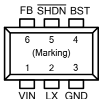
Figure 1. Pin Assignments of FR9206F
