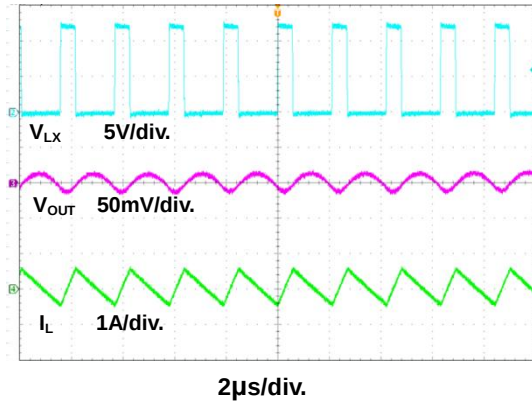
Figure 15. Steady State Waveform
