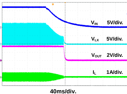
Figure 19. Power Off Through VIN Waveform
