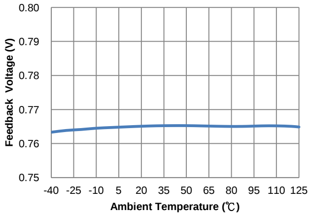
Figure 13. Feedback Voltage vs. Ambient Temperature
