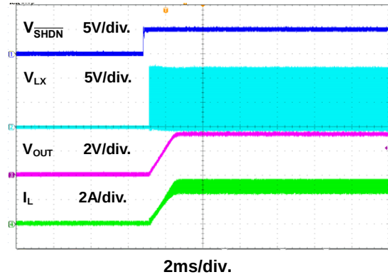
Figure 22. Power On Through \overline{SHDN} Waveform
