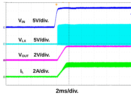
Figure 18. Power On Through VIN Waveform
