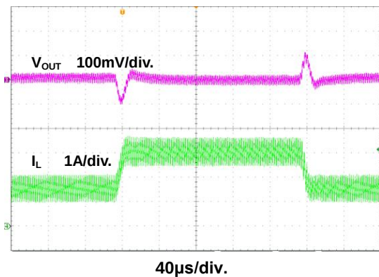
Figure 25. Load Transient Waveform
