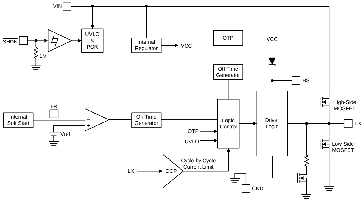
Figure 4. Block Diagram of FR9206F
