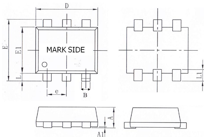
SOT-563-6 Package (Unit: mm)
