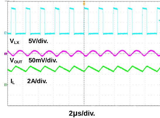
Figure 16. Steady State Waveform
