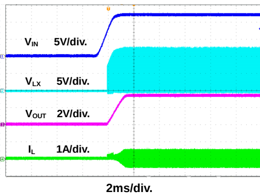
Figure 17. Power On Through VIN Waveform
