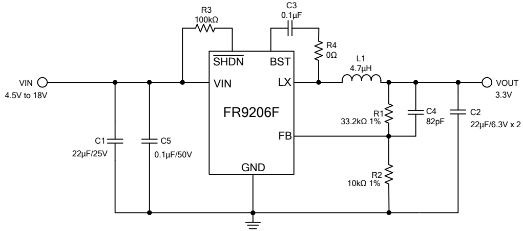
Figure 2. FR9206FS9 Application Circuit
