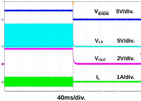
Figure 23. Power Off Through \overline{SHDN} Waveform
