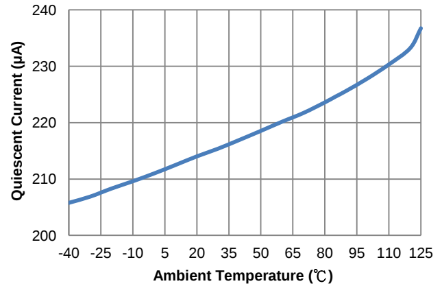
Figure 12. Quiescent Current vs. Ambient Temperature
