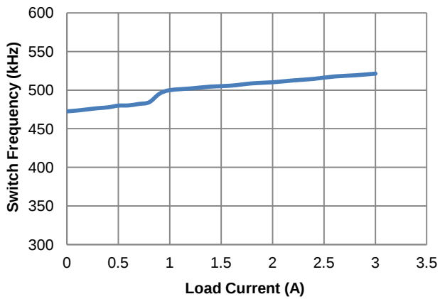
Figure 11. Switch Frequency vs. Load Current
