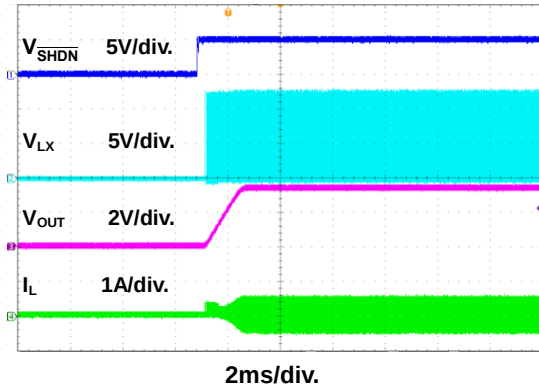
Figure 21. Power On Through \overline{SHDN} Waveform
