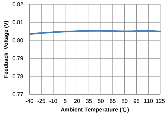
Figure 14. Feedback Voltage vs. Ambient Temperature
