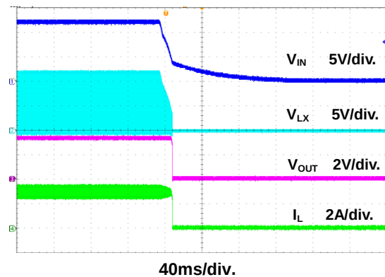
Figure 20. Power Off Through VIN Waveform
