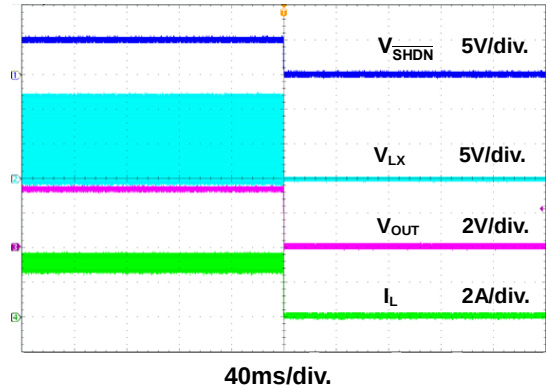
Figure 24. Power Off Through \overline{SHDN} Waveform
