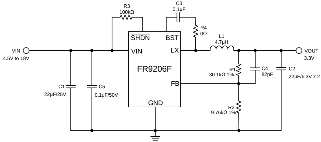
Figure 3. FR9206FSD Application Circuit
