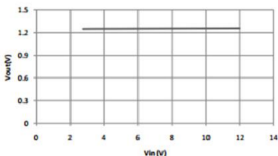
1117C-ADJ V_{\text{out}} Vs. V_{\text{in}}
