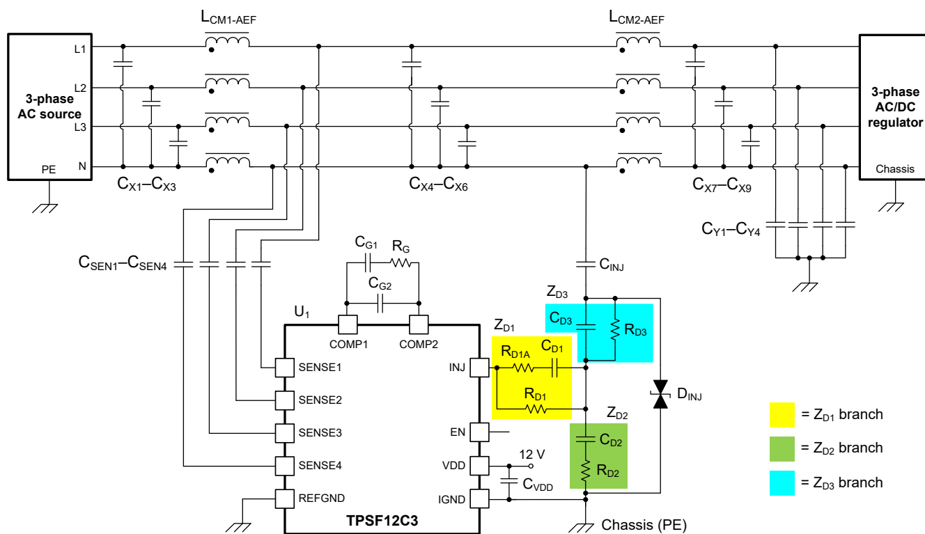
Figure 9-3. Injection Network
