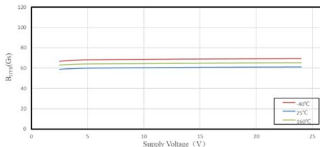
SC2443 B_{HYS} VS. Supply Voltage
