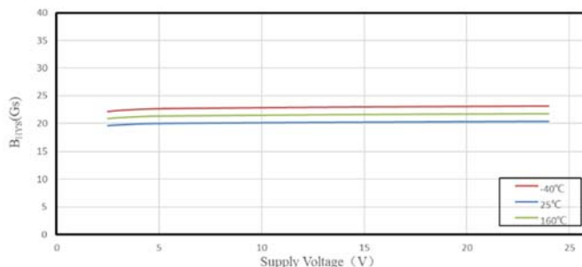
SC2440 B_{HYS} VS. Supply Voltage
