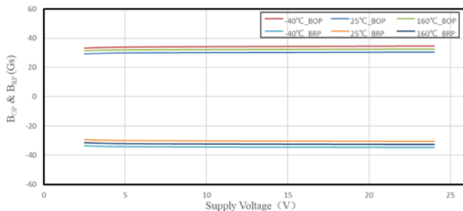
SC2443 B_{OP} & B_{RP} VS. Supply Voltage
