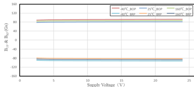
SC2448 B_{OP} & B_{RP} VS. Supply Voltage
