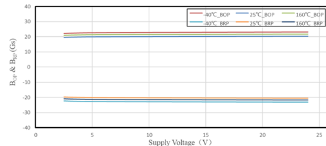
SC2442 B_{OP} & B_{RP} VS. Supply Voltage
