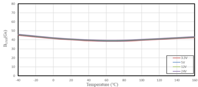
SC2442 B_{HYS} VS. Temperature
