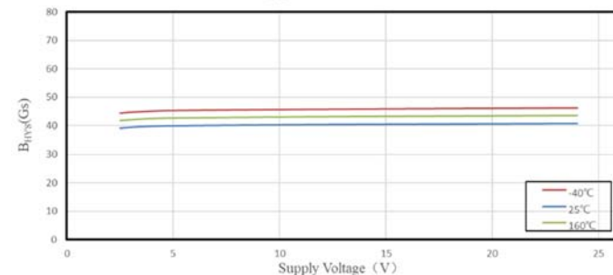
SC2442 B_{HYS} VS. Supply Voltage
