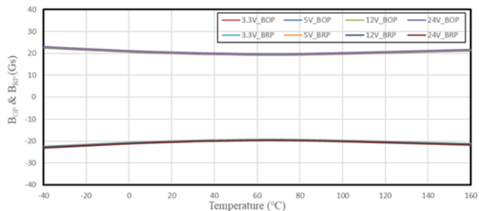
SC2442 B_{OP} & B_{RP} VS. Temperature
