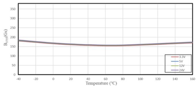
SC2448 B HYS VS. Temperature
