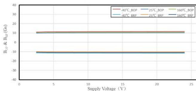
SC2440 B OP & B RP VS. Supply Voltage
