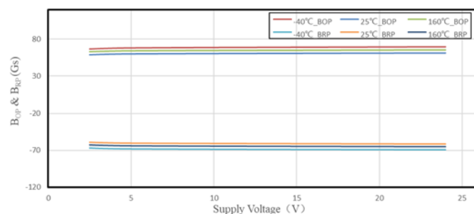
SC2446 B_{OP} & B_{RP} VS. Supply Voltage
