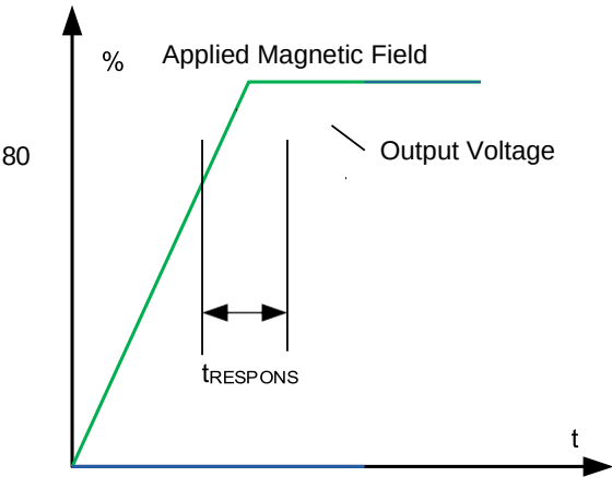
Figure 2. Response Time
