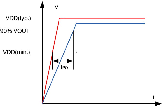
Figure 1. Power-On Time
