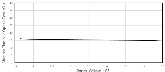
|B_{RP}| VS. Supply Voltage
