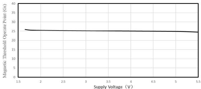
|B_{OP}| VS. Supply Voltage
