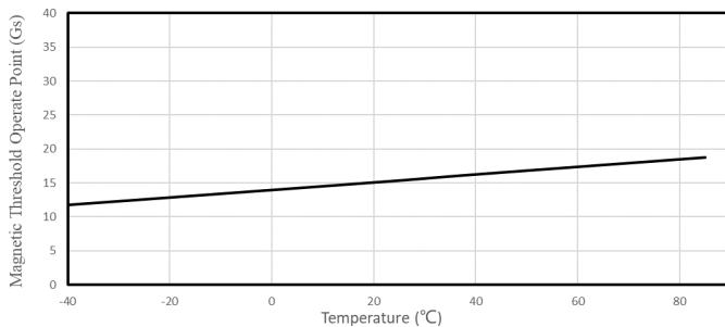
|B_{RP}| VS. Temperature
