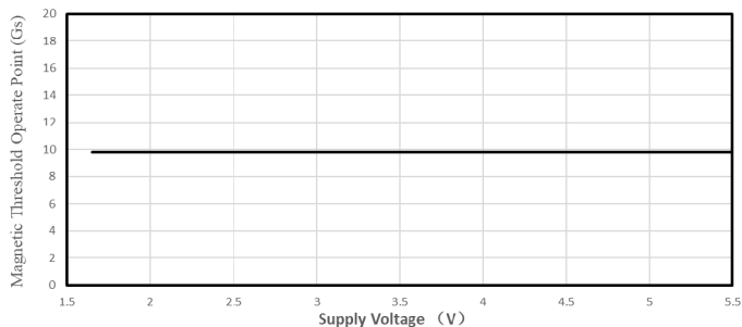
|B_H| VS. Supply Voltage
